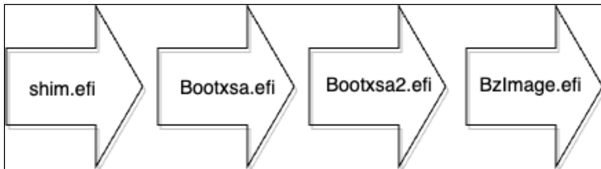
Figure 37: VSS UEFI Boot Sequence
