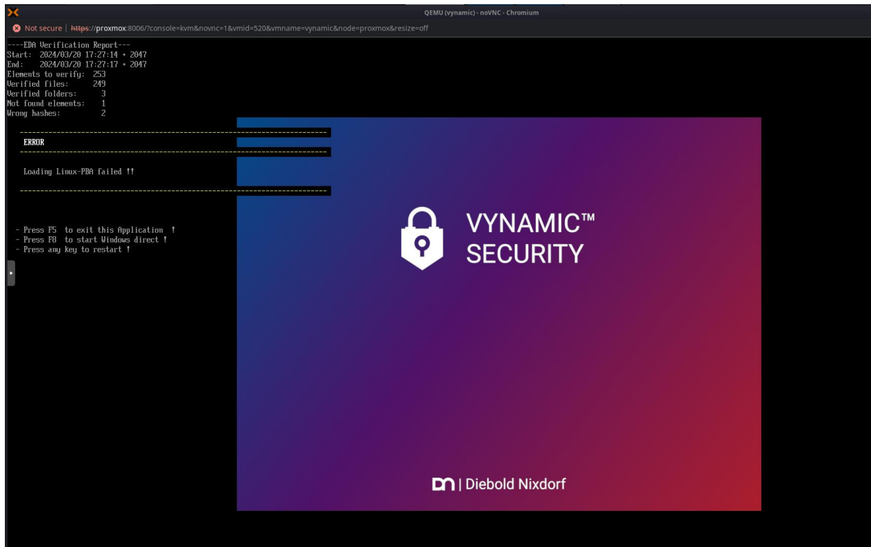
Figure 20: VSS - PBA Integrity Failure
