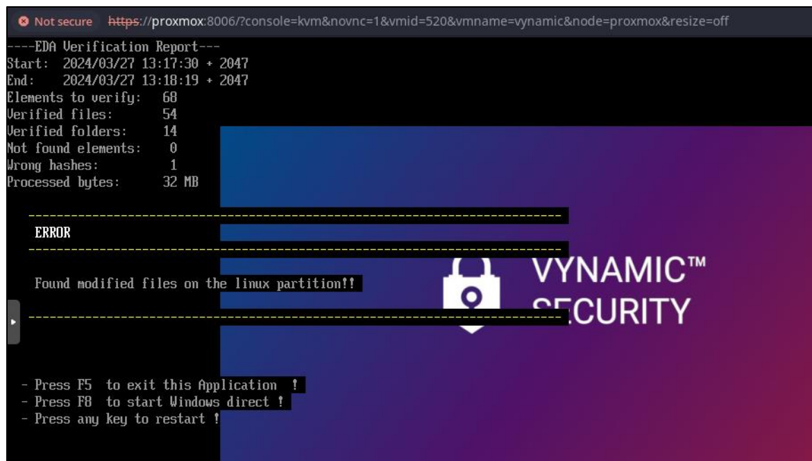
Figure 92: VSS v3.3.0 SR15 - PBA Phase I Failure on Empty File
