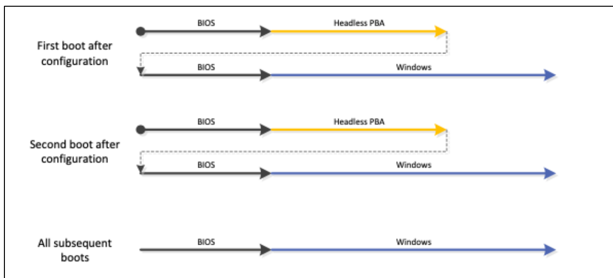
Figure 6: VSS FDE – PBA Boot Sequence
