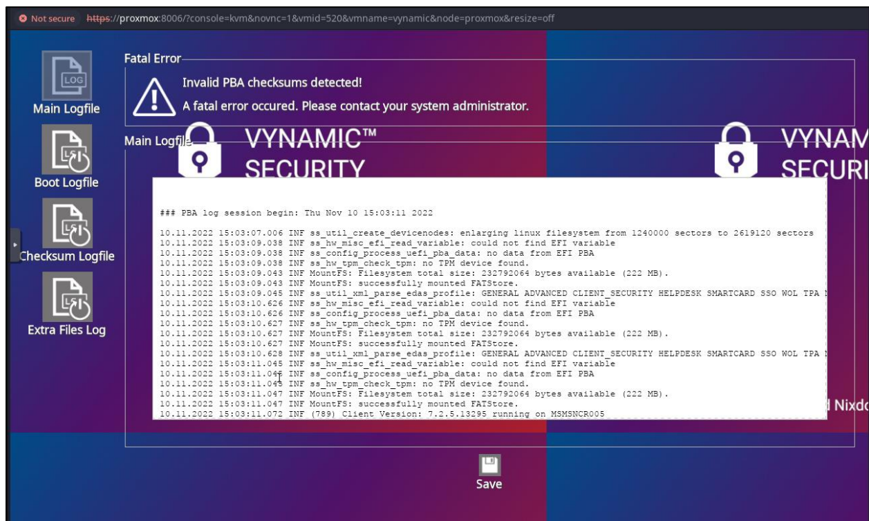
Figure 19: VSS PBA Error - wc Modification
