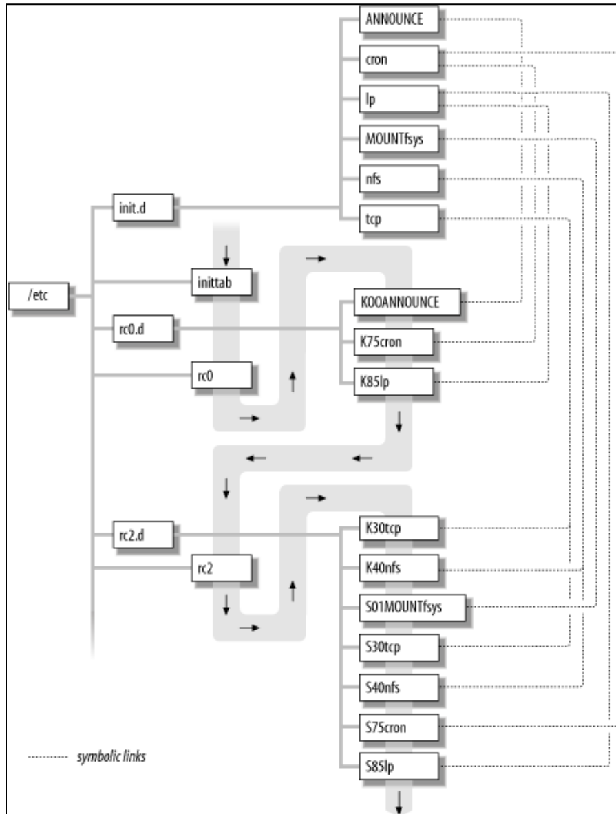
Figure 41: Essential System Administration, 3 rd Edition – Executing System V-style Boot Scripts
