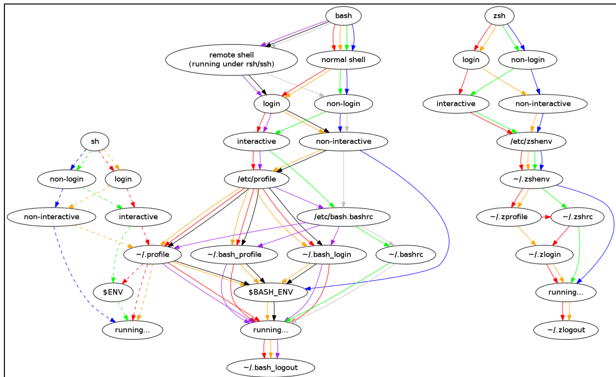
Figure 46: Linux BASH - Login Initialization Process
