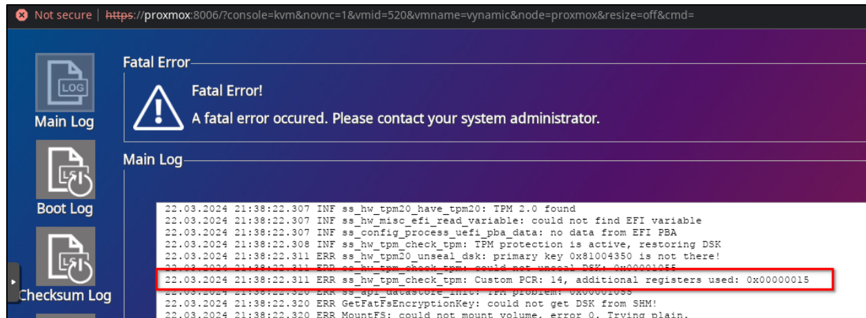
Figure 27: VSS TPM PCR 14 Error
