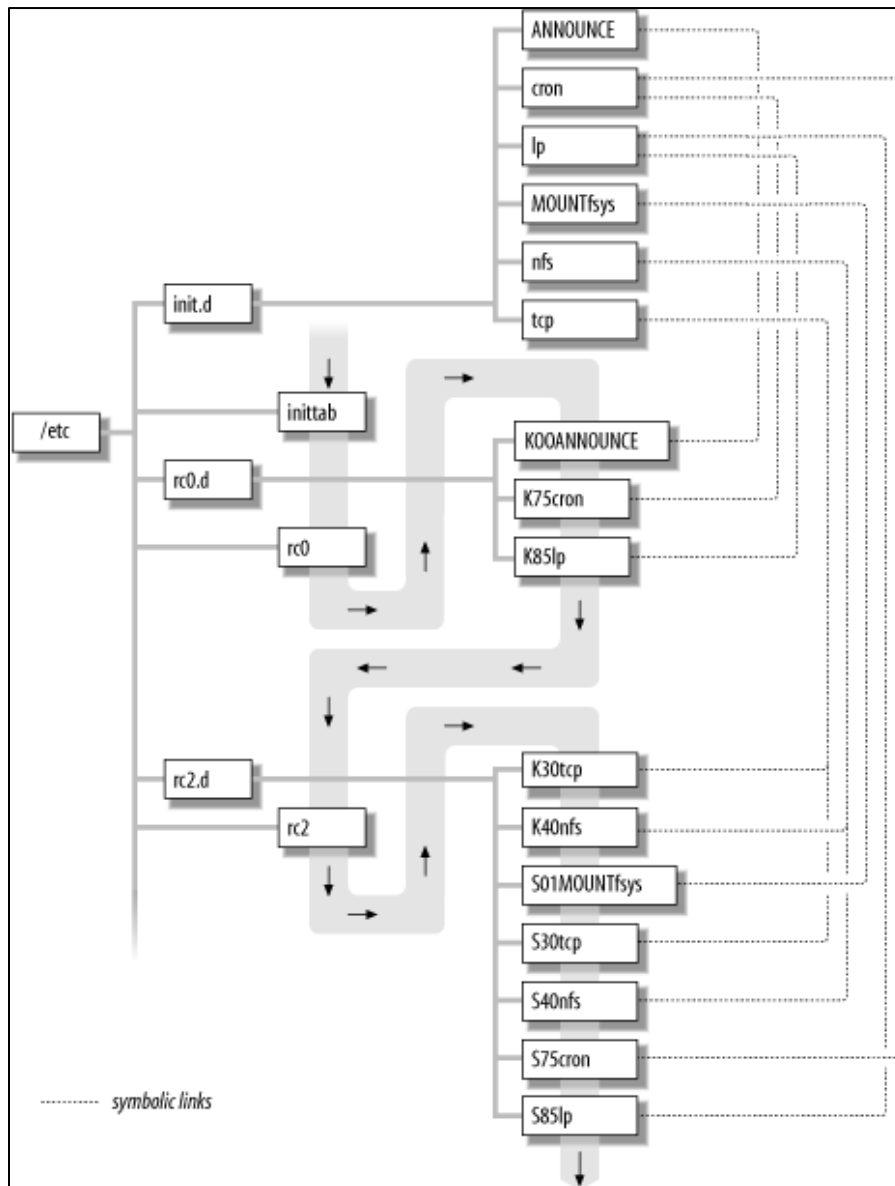
Figure 70: Essential System Administration, 3 rd Edition – Executing System V-style Boot Scripts
